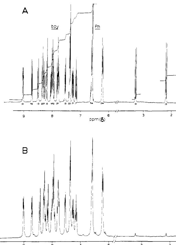
Figure 1. ^1\text{H NMR} spectrum in \text{CD}_2\text{Cl}_2 of (a) [\text{cis-Ru}(\text{bpy})_2(\text{CO})(\eta\text{-CH}_2\text{Ph})](\text{PF}_6) and (b) [\text{cis-Ru}(\text{bpy})_2\text{CO}(\eta\text{-CD}_2\text{Ph})](\text{PF}_6) isolated as the product of the reaction in \text{D}_2\text{O} (99.5%); see text. \text{Me}_4\text{Si} and methylene chloride peaks are deleted.
